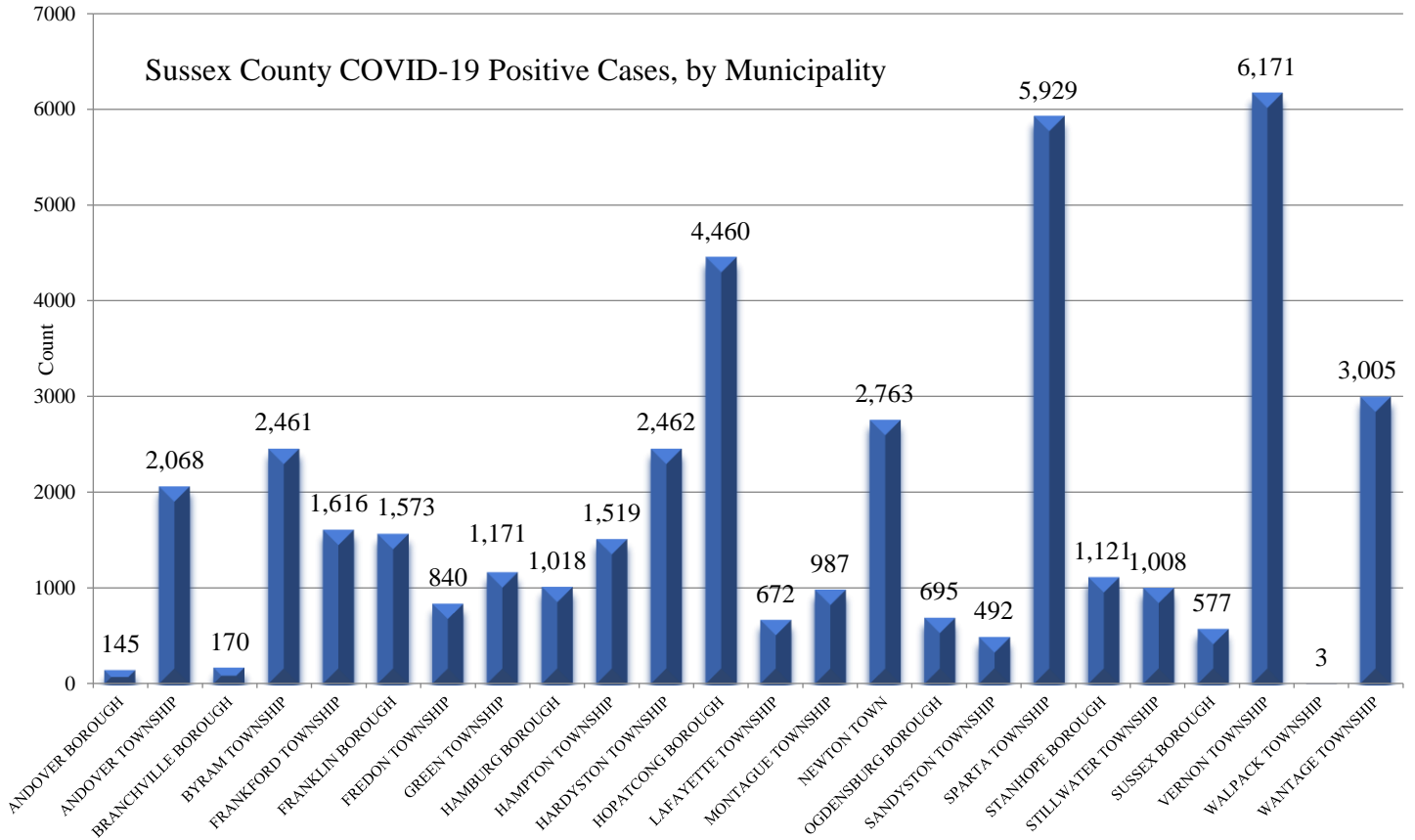
Figure 1: Sussex County Total COVID-19 Cases by Municipality
