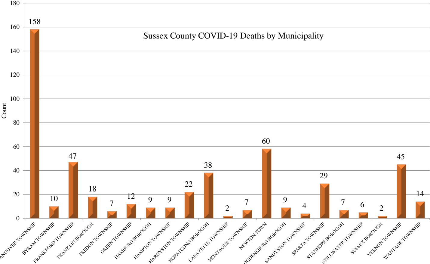
Figure 6: Sussex County COVID-19 Deaths by Municipality
