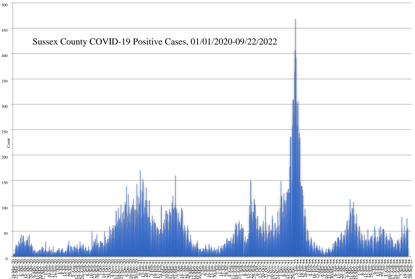
Figure 2: Sussex County Positive COVID-19 Cases by Reported Date
